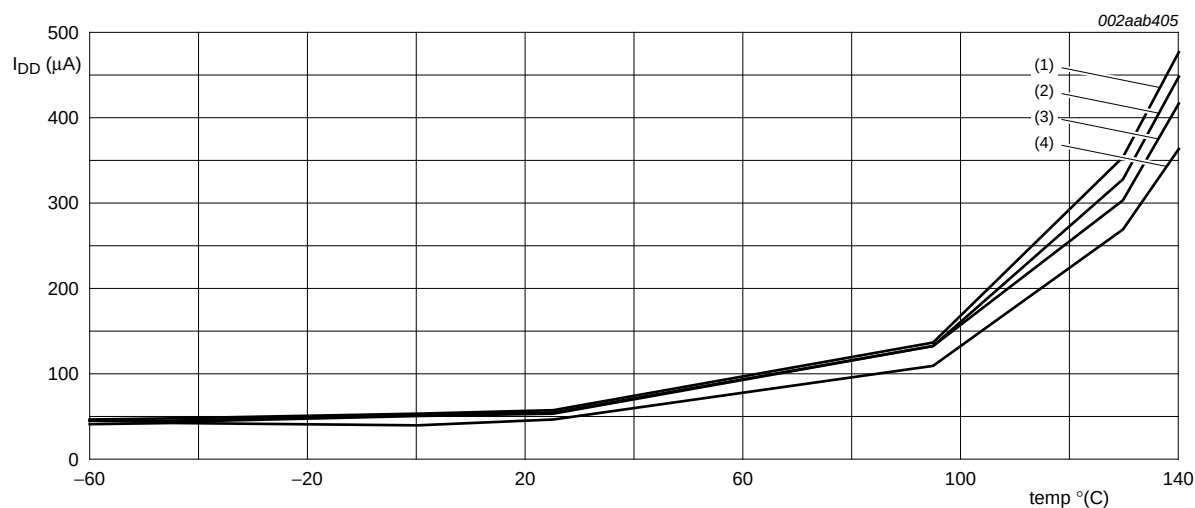
Fig 10. I_{DD(pd)} measured at different temperatures
