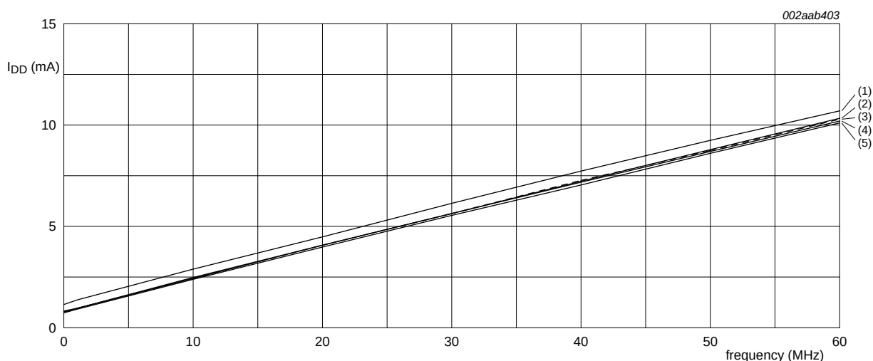
Fig 9. I_{DD} idle measured at different frequencies (CCLK) and temperatures
